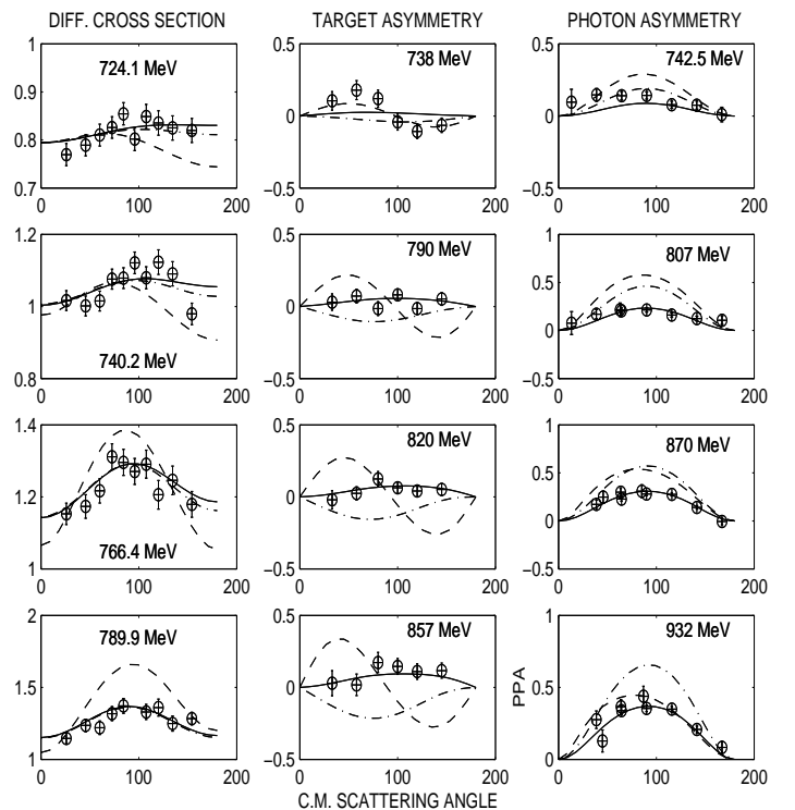
FIG. 1. Differential cross-section and polarization observables in our effective Lagrangian fit with different choices of energy segments. Solid : Fitting Mainz [4], Bonn [5] and GRAAL [6] data upto 790, 895 and 932 MeV respectively; dash-dot: fitting Mainz data alone; dash: fitting a low-energy truncation of the Mainz and Bonn data, upto 750 MeV.
